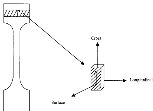
Fig.1. Schematic diagram of samples taking from a test specimen and the three directions.
