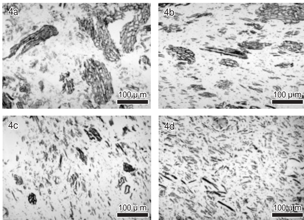
Fig. 4 Optical microphotographs of cross sections. a: Sample 2, b: Sample 3, c: Sample 4, d: Sample 5.
