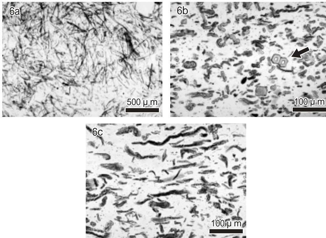
Fig. 6 Optical microphotographs of Sample 6. a: thin layer, b: cross section, c: longitudinal section. arrow : contaminations of coniferous tracheids.
