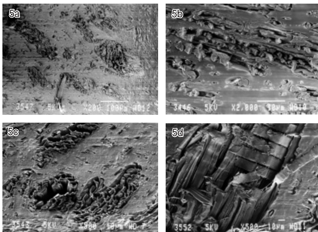
Fig. 5 SEM micrographs of microtome-planned blocks. a, c & d: Sample 3, b: sample 5. a--c: longitudinal section, d: surface section. a & b: untreated, c & d: treated for complete removal of cell wall materials.
