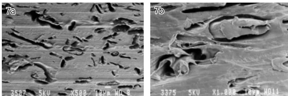
Fig. 7 SEM micrographs of Sample 6 treated to remove cell wall material. a: cross section, b: longitudinal section.
