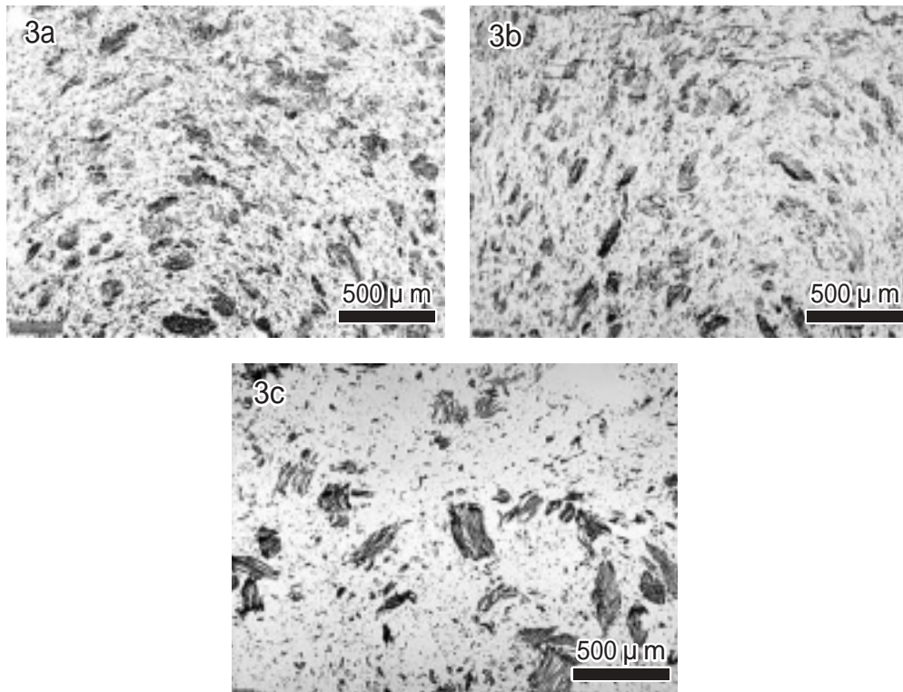
Fig. 3 Optical microphotographs of Sample 2. a: cross section, b: longitudinal section, c: surface section.
